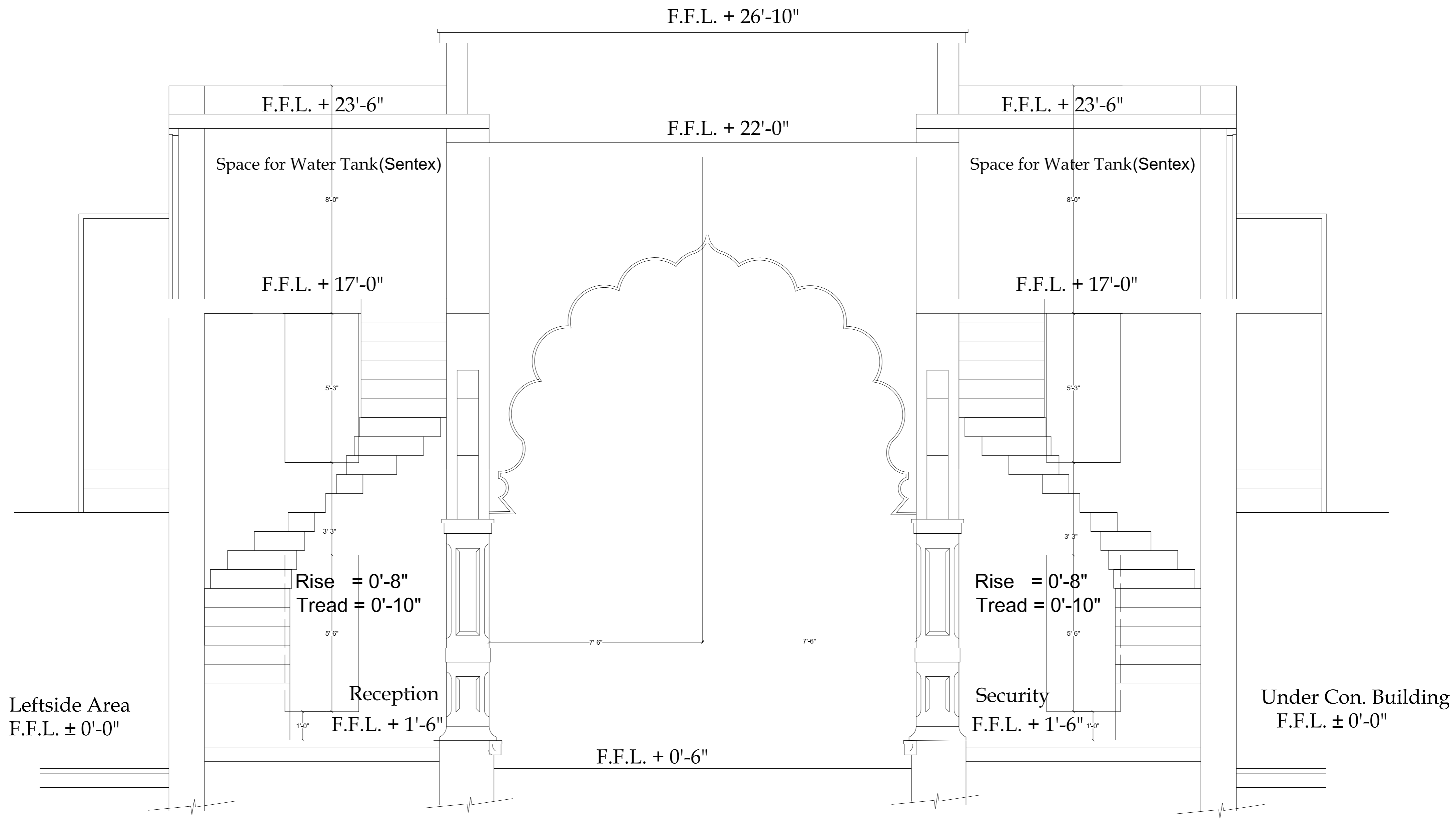
Section at "B-B"
